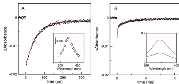
Figure 1. Flash-photolysis measurements of Ty oxy by 355 nm pulse irradiation. Absorbance changes at 345 nm under (A) 100% O 2 and (B) O 2 :CO = 1:1 (v/v). (A) Single and (B) double exponential best-fitted curves are shown in red. Experimental conditions: Ty, 20 \mu M; O 2 , (A) 1.54 mM and (B) 0.77 mM; 15 °C; 50 mM potassium phosphate buffer, pH 7.2; laser pulse, 30 mJ, 10 Hz. The traces are an average of (A) 128 and (B) 256 shots. (Inset) A: Overlap of wavelength dependence of the initial absorbance changes (empty circles) with the difference absorption spectrum (red, oxy minus deoxy). B: Absorption spectra of Ty under 100% O 2 (red) and O 2 :CO = 1:1 (v/v) (blue).
